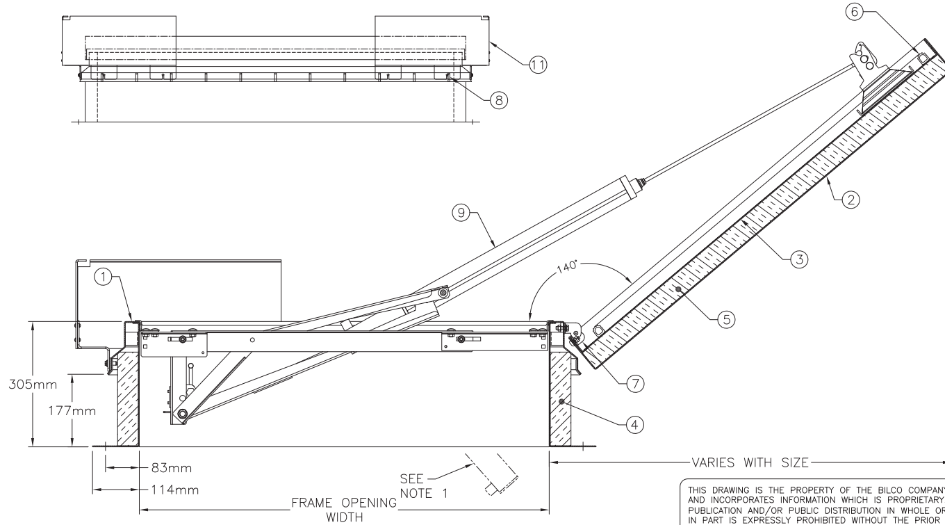
SECTION
