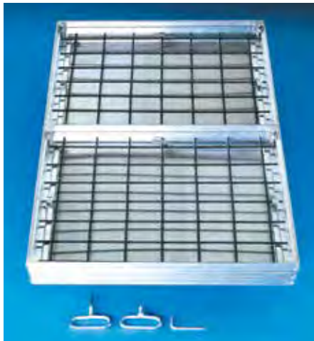
BVA Multi Aluminium Pan Depth: 66mm Load Capacity: 125kN Test Load EN 124
