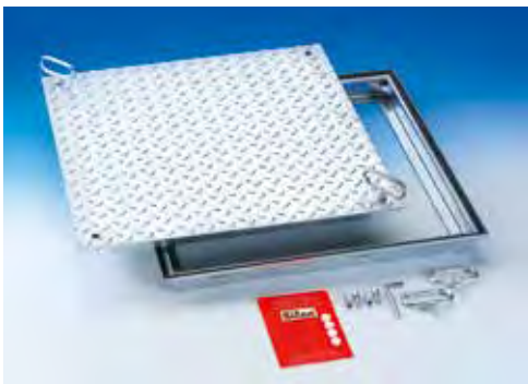
RV Galvanised Steel RVE Stainless Steel Load Capacity: 15kN Test Load EN 124
