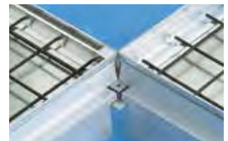
Connection of cover assemblies
