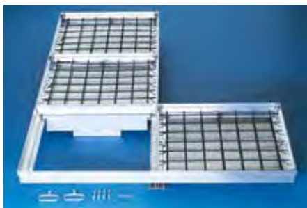
BVA-RA Aluminium Pan Depth: 66mm Load Capacity: 125kN Test Load EN 124
